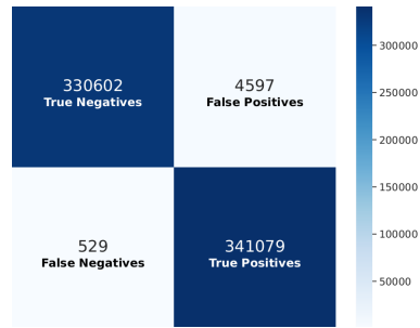
(c) The confusion matrix for 1D-CNN.
