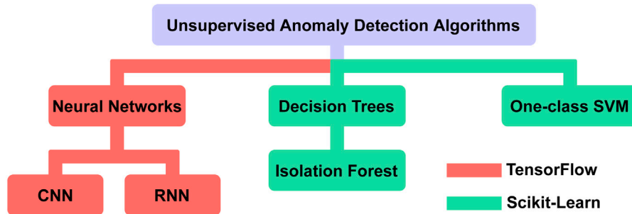
Fig. 1. Illustrates the utilized algorithms. TensorFlow also has an API [27] for decision trees, but due to having better documentation we prefer using scikit-learn for implementing Isolation Forest.
