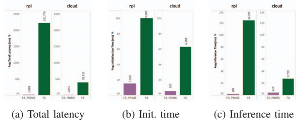
Fig. 9: Comparison: F3 and F3_PRIME
