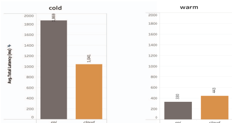
Fig. 10: Average latency: F3_PRIME in cold/warm activation
